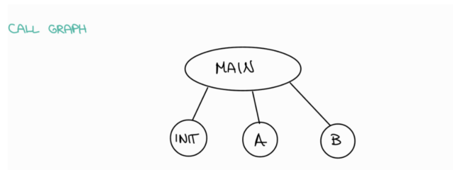
Figura 3.24: Call Graph
